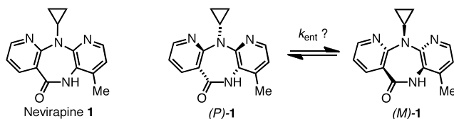
Figure 1: Nevirapine and its enantiomeric conformers
