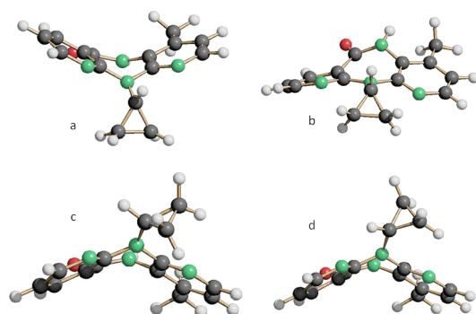
Figure 4. The global minimum (a), the inversion transition state (b), the local minimum (c) and the transition state from the local minimum to the global minimum (d).
