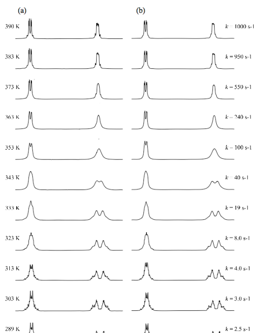
Figure 3: (a) Experimental and (b) modelled bandshapes for H_A – H_X .
